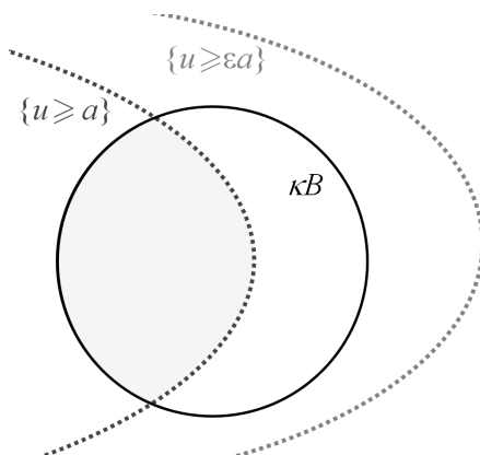
Figure 8.1. Level sets \{u \geq a\} and \{u \geq \varepsilon a\} .
