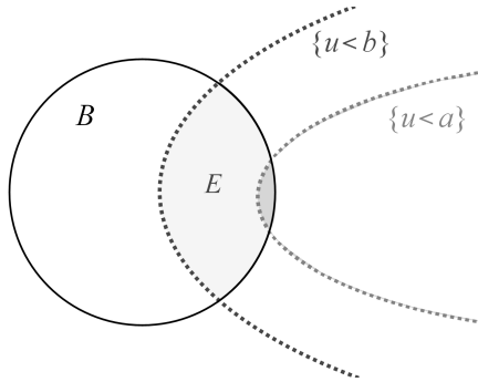
Figure 6.2. Set E = B \cap \{u < b\} .
