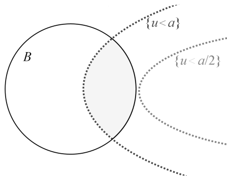
Figure 6.1. Level sets \{u < a\} and \{u < a/2\} .
