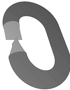
Figure 1.1. The light coloured part of the boundary carries Dirichlet boundary conditions, the dark coloured part has Neumann boundary conditions.
